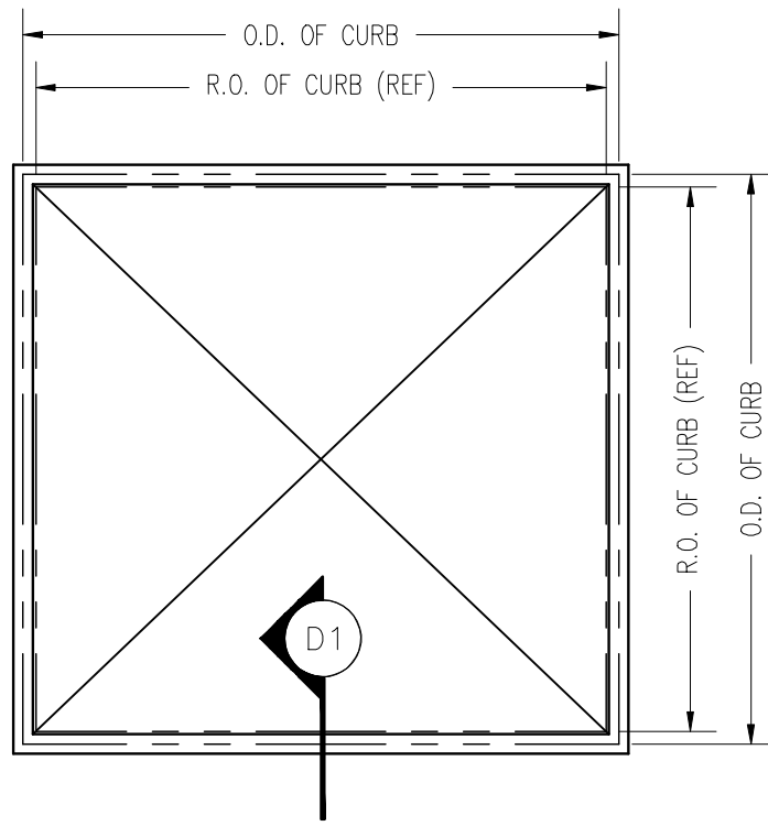
PYRAMID GLAZING SHOWN – CURVED GLAZING SIMILAR
